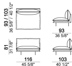
Composition "C" (left unit 246x103 cm + left corner sofa 261x103 cm)
