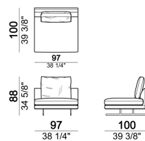
Central unit, back cushion 70 cm
