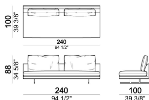
Central unit, back cushions 100 cm
