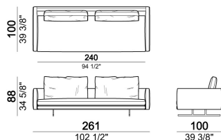
Sofa, back cushions 70 cm
