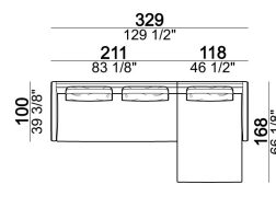
Composition "A" (left unit 211 cm + chaise-longue 118x168 cm with right short arm, 3 back cushions 80 cm)
