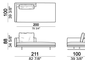
Unit with right or left pouf, back cushion 80 cm
