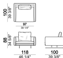
Sofa, back cushions 90 cm
