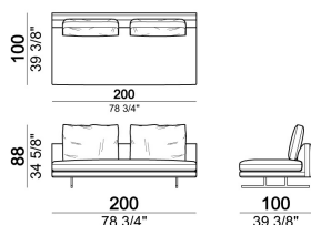
Central unit, back cushions 80 cm
