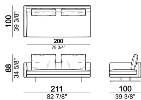
Right or left unit, back cushions 80 cm
