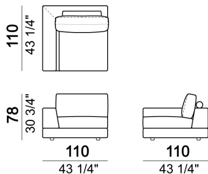
Relax unit type A 110 cm with right or left full arm
