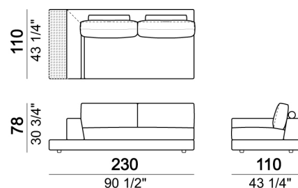
Unit with right or left arm and plat
