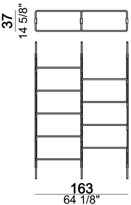
Ceiling bookshelf "3-01C " (3 uprights C + 1 bottom shelf 80T + 8 shelves 80 + 1 foot F).
