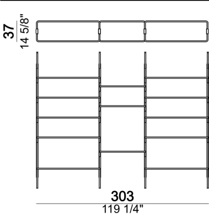
Ceiling bookshelf "4-02C " (4 uprights C + 2 bottom shelves 110T + 3 shelves 80 + 8 shelves 110).
