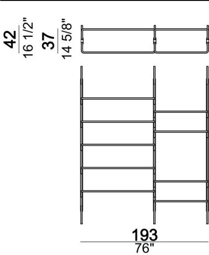
Wall bookshelf "3-02W " (3 uprights W + 1 bottom shelf 80T + 3 shelves 80 + 5 shelves 110 + 1 foot F).
