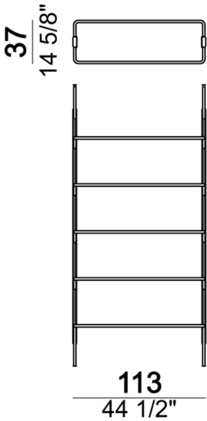
Ceiling bookshelf "2-03C " (2 uprights C + 1 bottom shelf 110T + 4 shelves 110).
