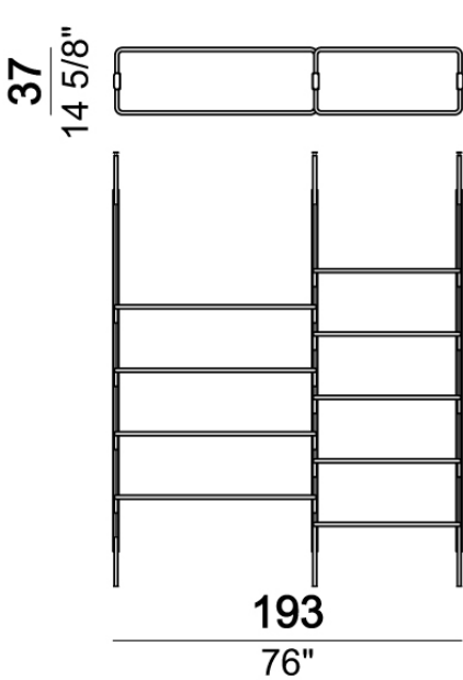
Ceiling bookshelf "3-05C " (3 uprights C + 1 bottom shelf 80T + 4 shelves 80 + 4 shelves 110 + 1 foot F).
