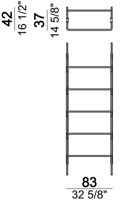
Wall bookshelf "2-01W " (2 uprights W + 1 bottom shelf 80T + 4 shelves 80).
