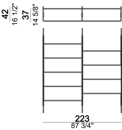
Wall bookshelf "3-04W " (3 uprights W + 1 bottom shelf 110T + 8 shelves 110 + 1 foot F).
