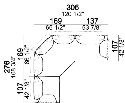
Composition C (left unit 107 cm + corner unit 169 cm + right unit 137 cm)
