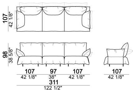
Sofa made by left unit 107 cm + central unit 97 cm + right unit 107 cm
