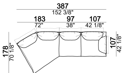
Composition E (dormeuse 183 cm with left angle 30° + central unit 97 cm + right unit 107 cm)
