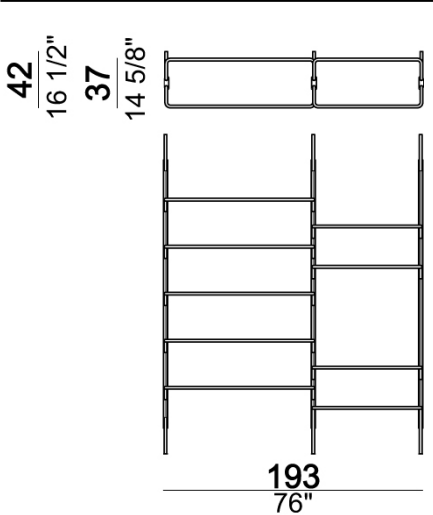
Wall bookshelf "3-02W " (3 uprights W + 1 bottom shelf 80T + 3 shelves 80 + 5 shelves 110 + 1 foot F).
