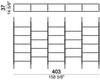
Ceiling bookshelf "6-01C " (6uprights C + 3 bottom shelves 80T + 20 shelves 80).
