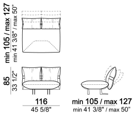
Central unit
