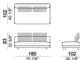
Central unit
