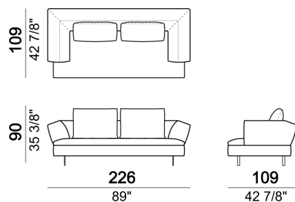
Sofa with back cushions 70 cm
