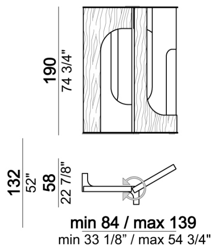
Floor room divider - 2 units
