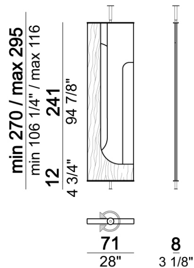
Ceiling room divider
