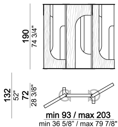
Floor room divider - 3 units
