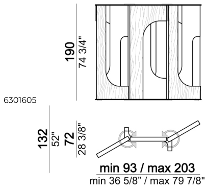
Floor room divider - 3 units
